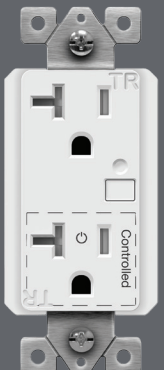
HALF-CONTROLLED 20A TAMPER-RESISTANT DECORATOR RECEPTACLE PL20R
